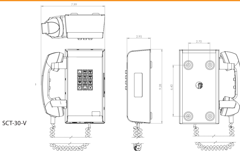
SCT-V Series Steel Compact VoIP Telephones
