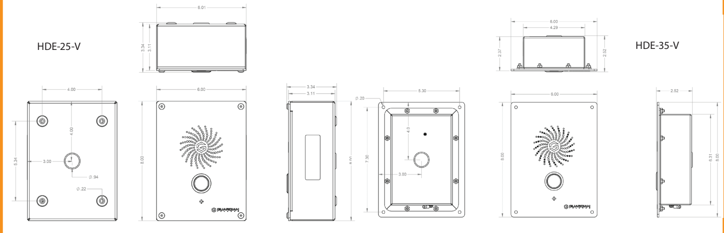
HDE-V COMPACT SERIES Heavy Duty Emergency & Public Access IP Telephones
