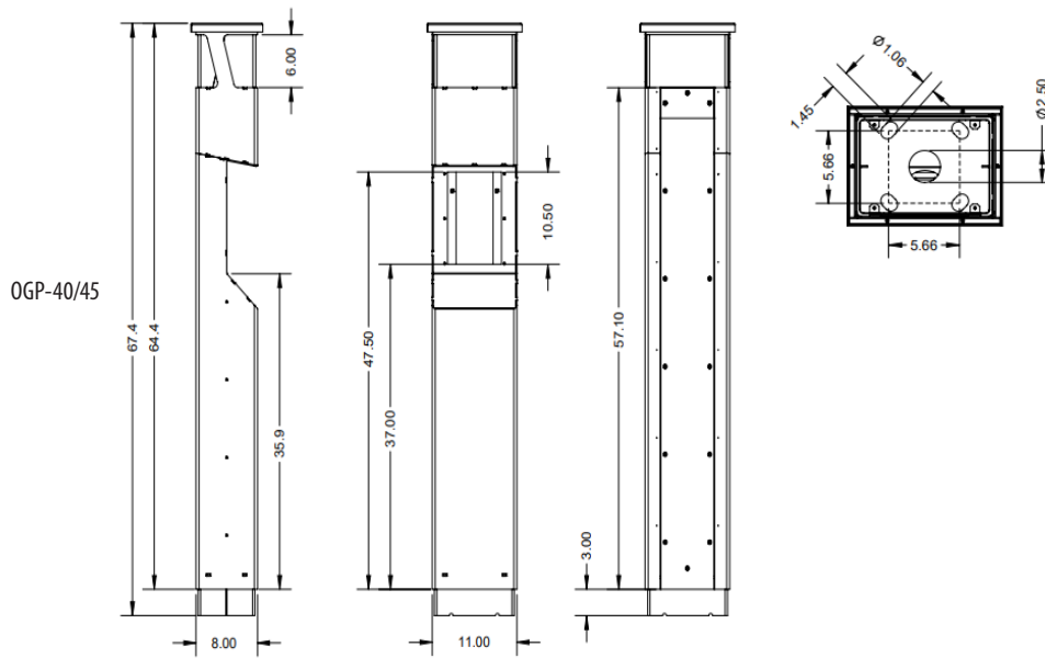
OGP 40/45 SERIES OUTDOOR HELP POINT TOWER
